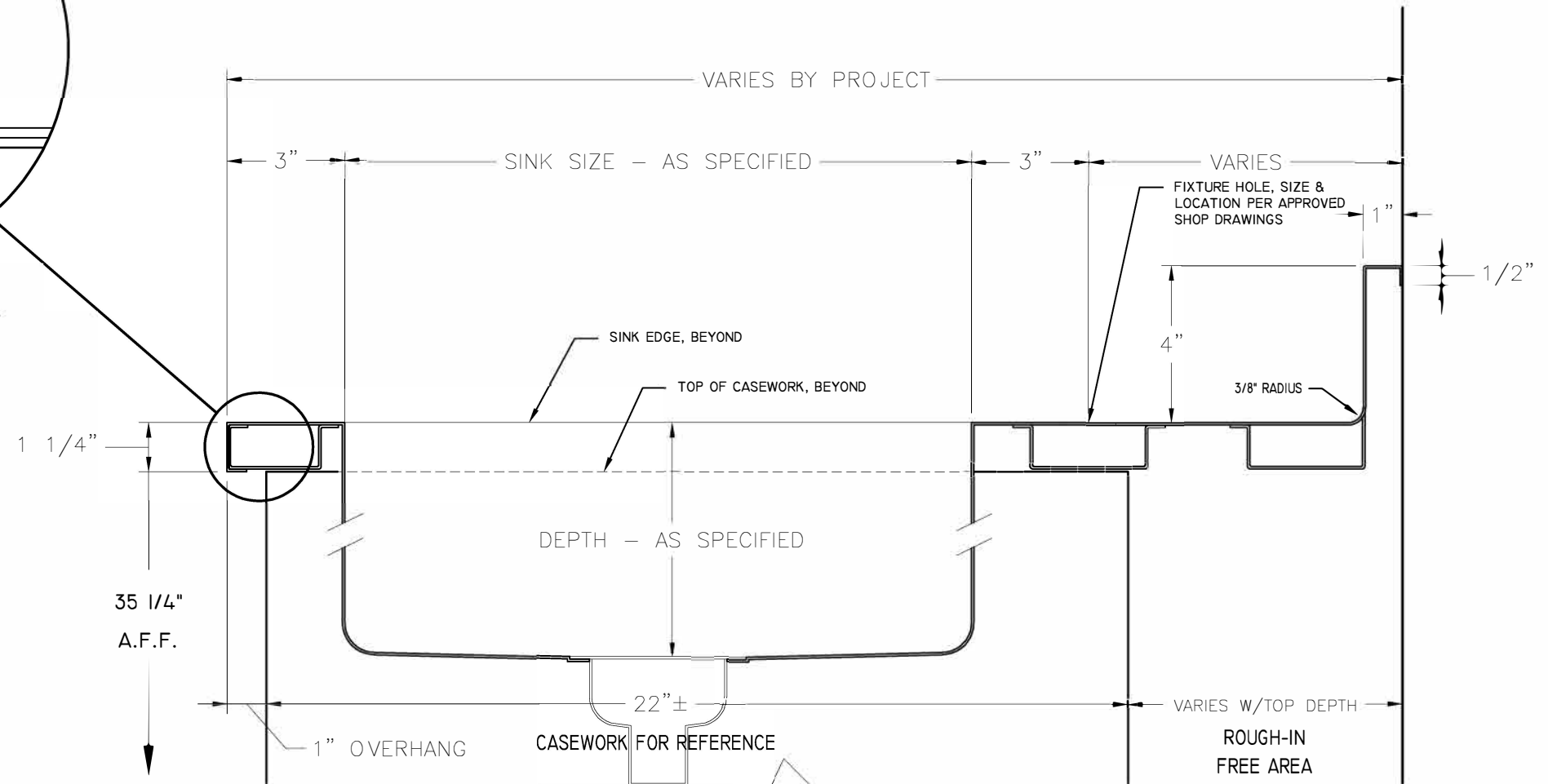
ENLARGED FRONT EDGE DETAIL
