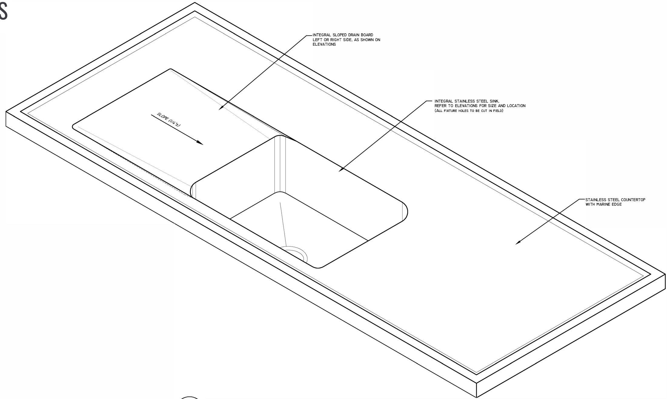
1 TYPICAL DRAIN BOARD @ STAINLESS STEEL COUNTER TOP WIDTH TO MATCH SINK, PITCH TO SINK W/OVERALL SLOPE OF 1/4"±
