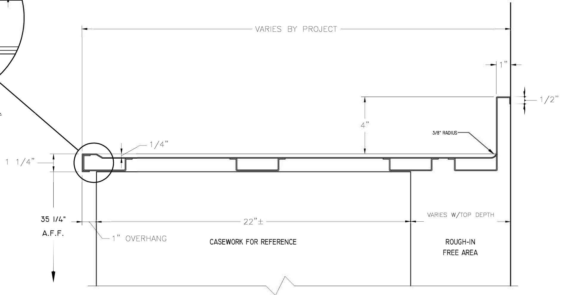
1 TYPICAL PERIMETER STAINLESS STEEL COUNTER TOP WITH MARINE EDGE AND HAT CHANNEL SUPPORT
