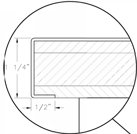
ENLARGED FRONT EDGE DETAIL
