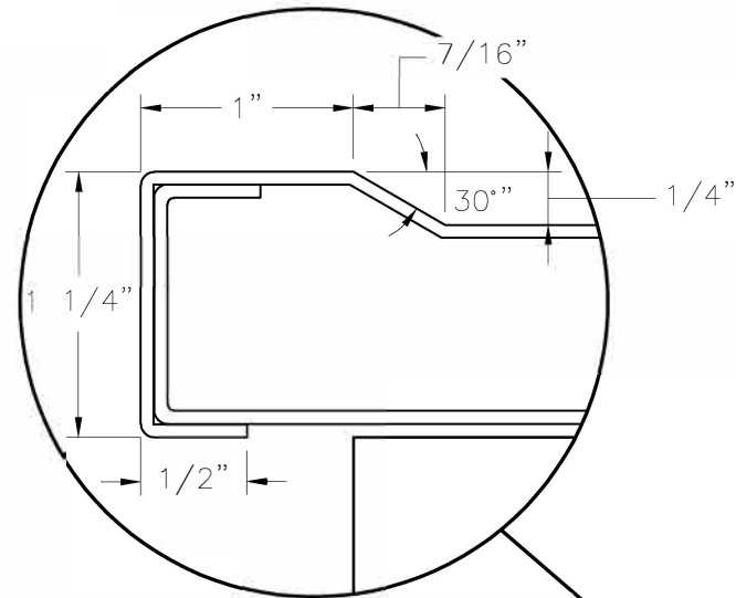
ENLARGED MARINE EDGE DETAIL
