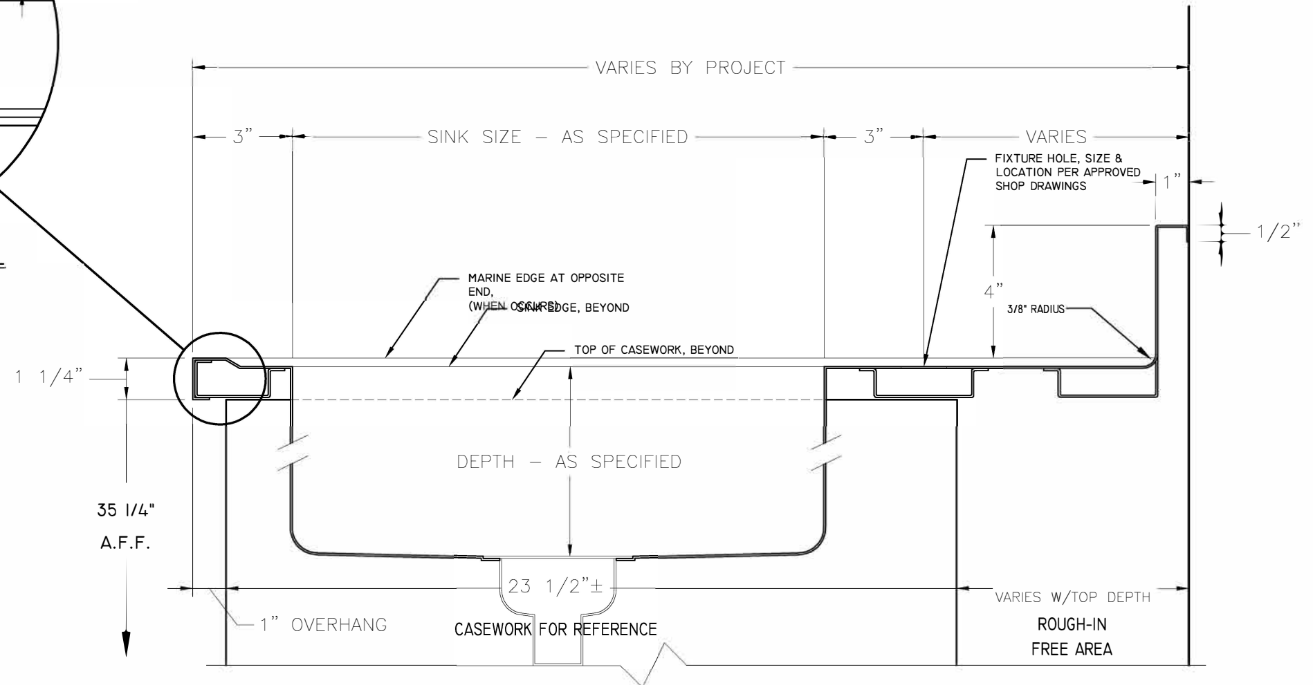
1 TYPICAL PERIMETER STAINLESS STEEL COUNTER TOP WITH MARINE EDGE, HAT CHANNEL SUPPORT, AND SINK
