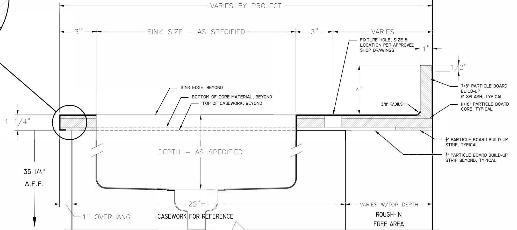
1 TYPICAL PERIMETER STAINLESS STEEL COUNTER TOP WITH PARTICLE BOARD CORE AND SINK
