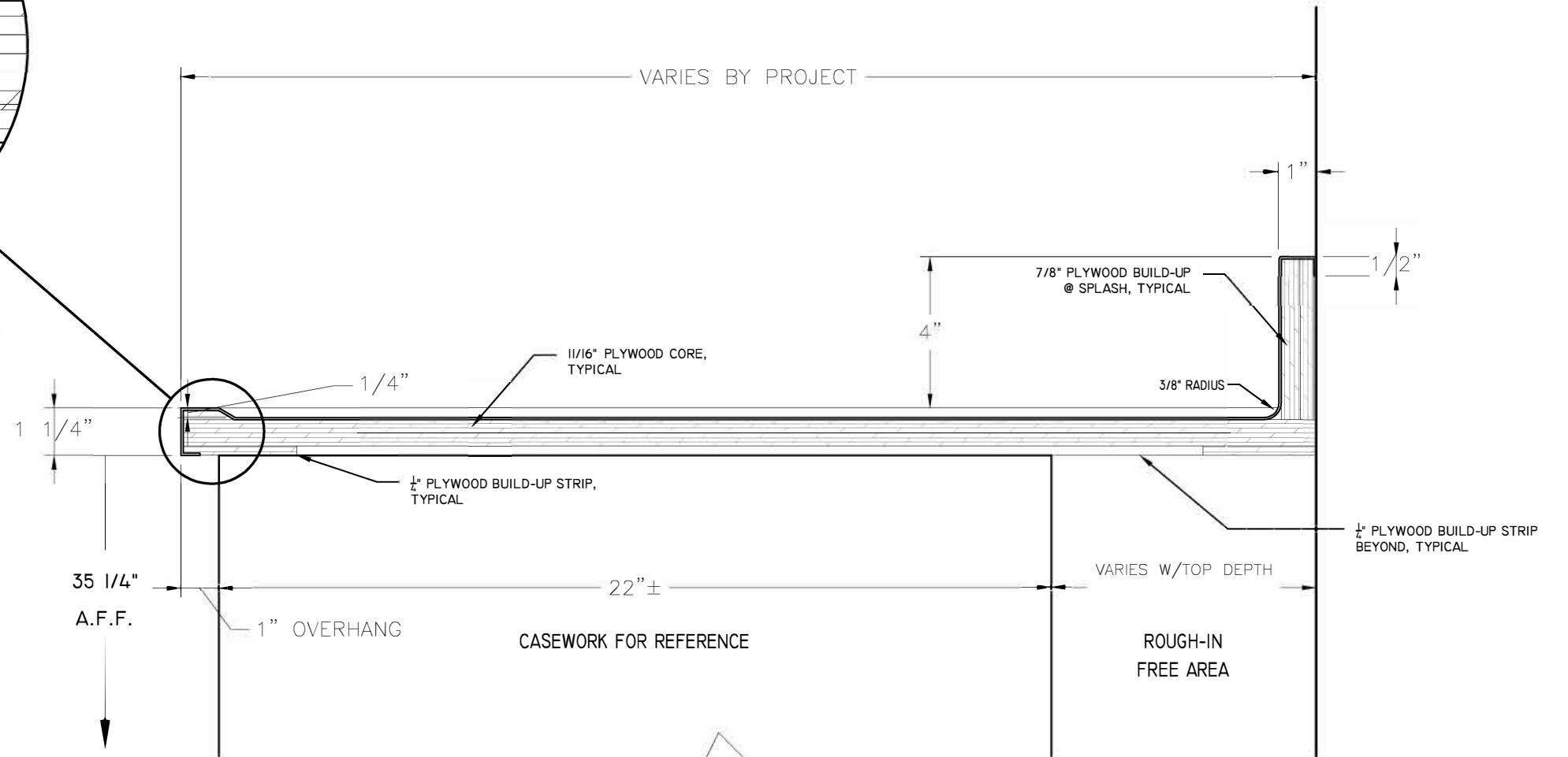
1 TYPICAL PERIMETER STAINLESS STEEL COUNTER TOP WITH MARINE EDGE AND PLYWOOD CORE
