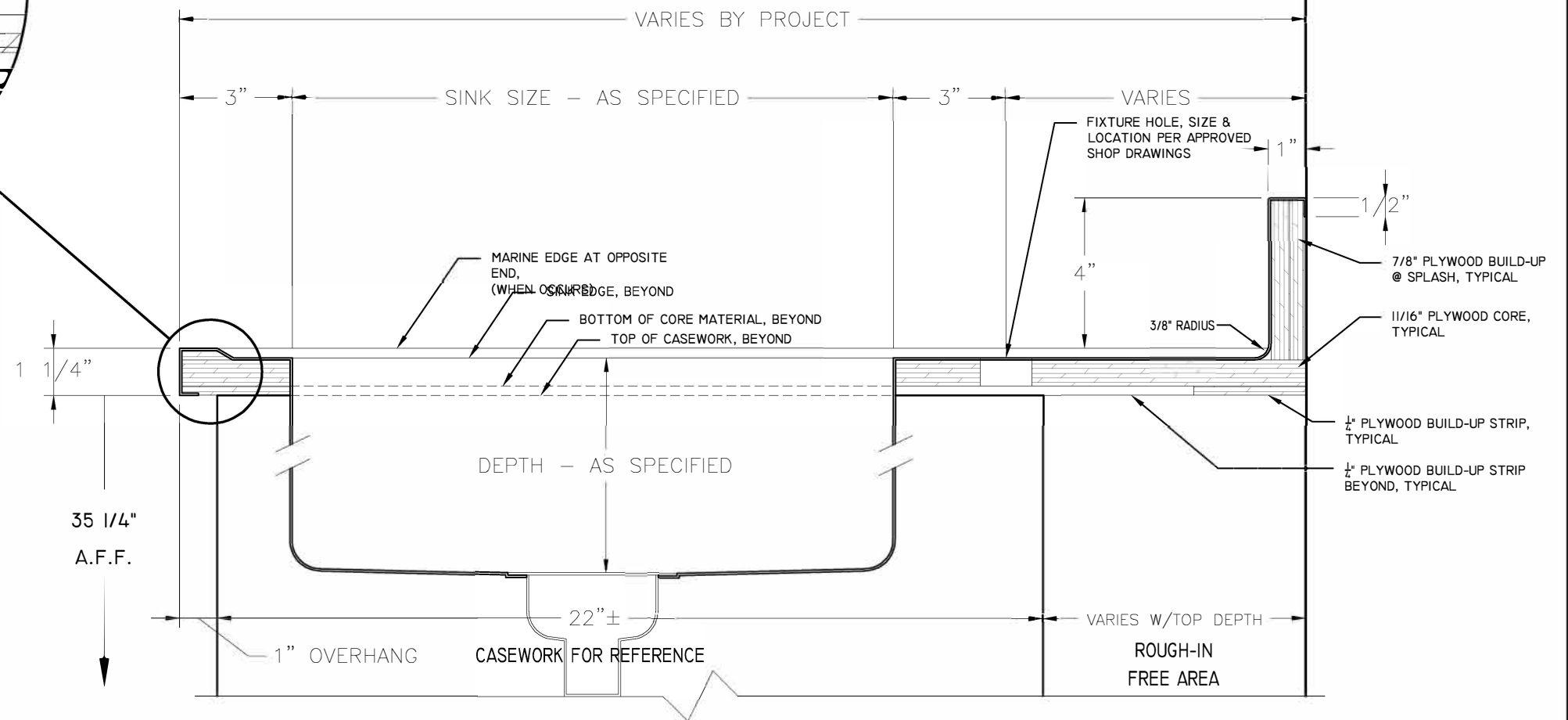
1 TYPICAL PERIMETER STAINLESS STEEL COUNTER TOP WITH MARINE EDGE, PLYWOOD CORE, AND SINK
