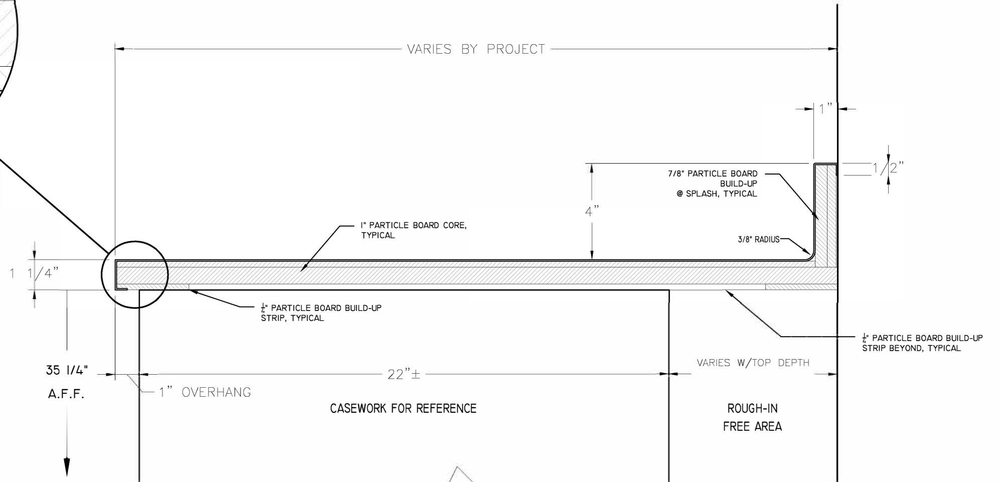
1 TYPICAL PERIMETER STAINLESS STEEL COUNTER TOP WITH PARTICLE BOARD CORE
