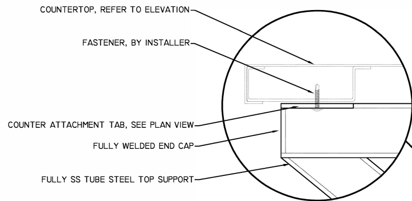
ENLARGED COUNTERTOP CONNECTION VIEW
