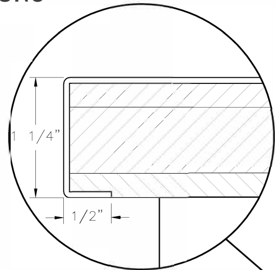
ENLARGED FRONT EDGE DETAIL
